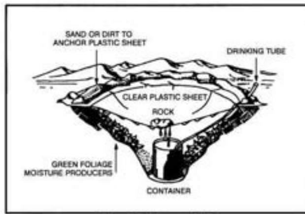
Figure 6-7. Belowground still.
