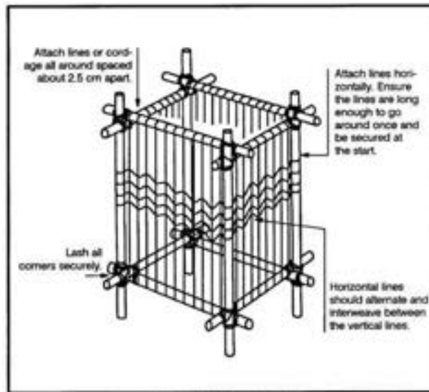
Figure 12-10. Square pack.
